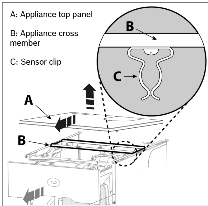
Fig. 1 Typical placement of the Fire Valve Sensor clip
